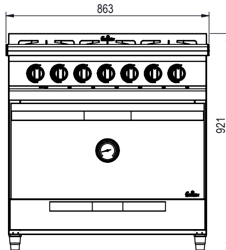
VISTA FRONTAL
